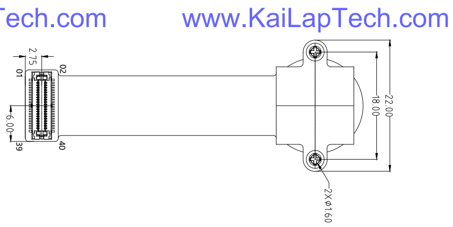
BOTTOM VIEW
